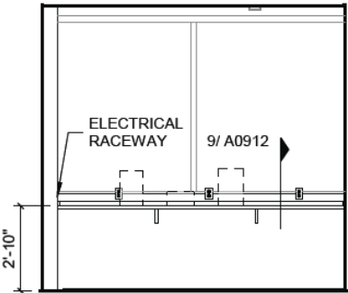
6 L03E BIO LAB PREP - EAST 1/4" = 1'-0" REF 1 / A0205
