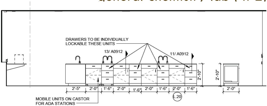
3 L04 GENERAL CHEMISTRY LAB - STUDENT 1/4" = 1'-0"
