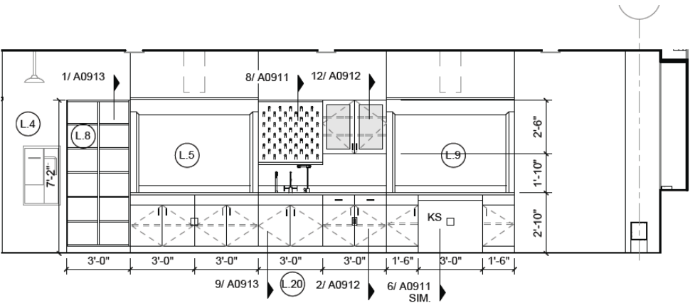
13 L04 ANALYTICAL/INORGANIC CHEM LAB - NORTH 1/4" = 1'-0"
