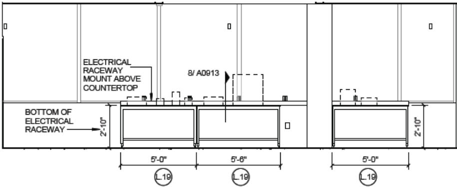
11 L02W CELL BIO AND PHYSICS RESEARCH - WEST 1/4" = 1'-0" REF 1 / A0204
