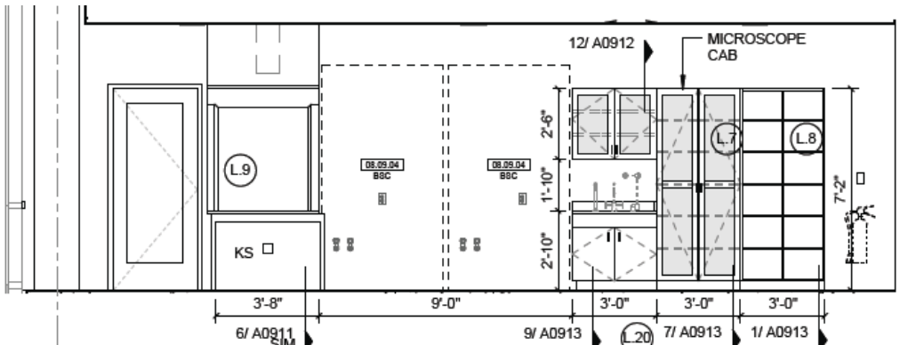
2 L03 CELL BIO / BIOCHEM LAB NORTH 1/4" = 1'-0"
