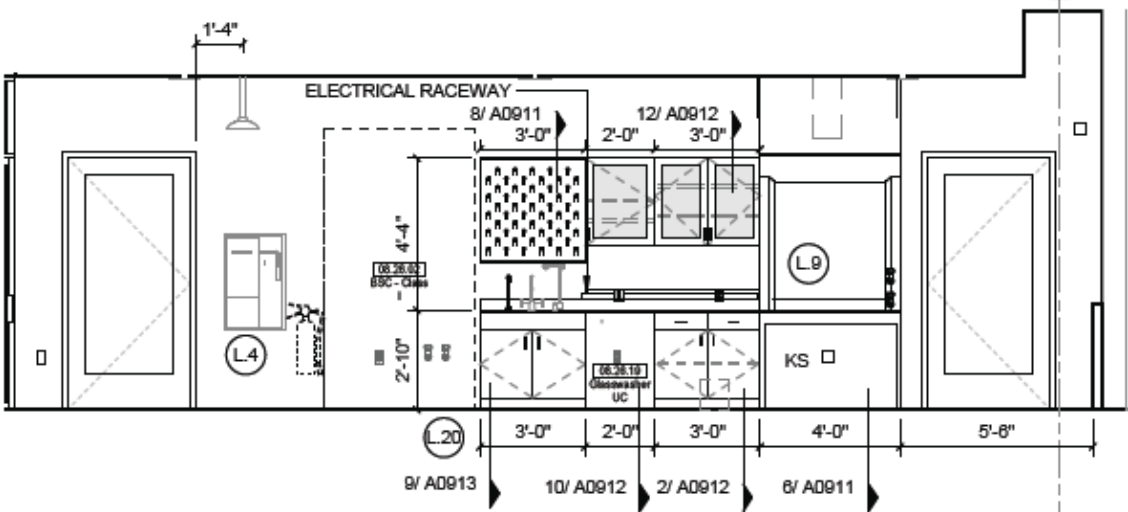
9 L02 CELL BIO / PHYSIO RESEARCH - SOUTH 1/4" = 1'-0"
