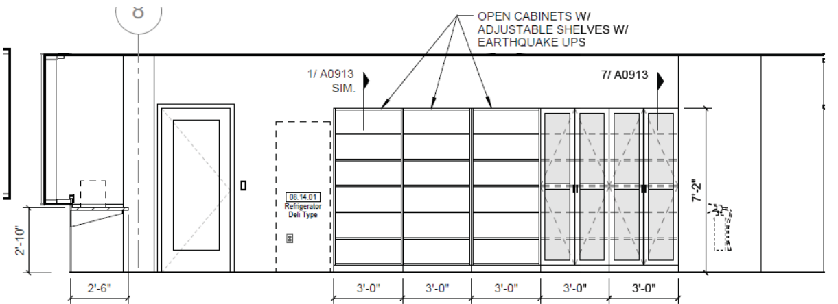
6 L04 CHEMISTRY LAB PREP - SOUTH 1/4" = 1'-0"
