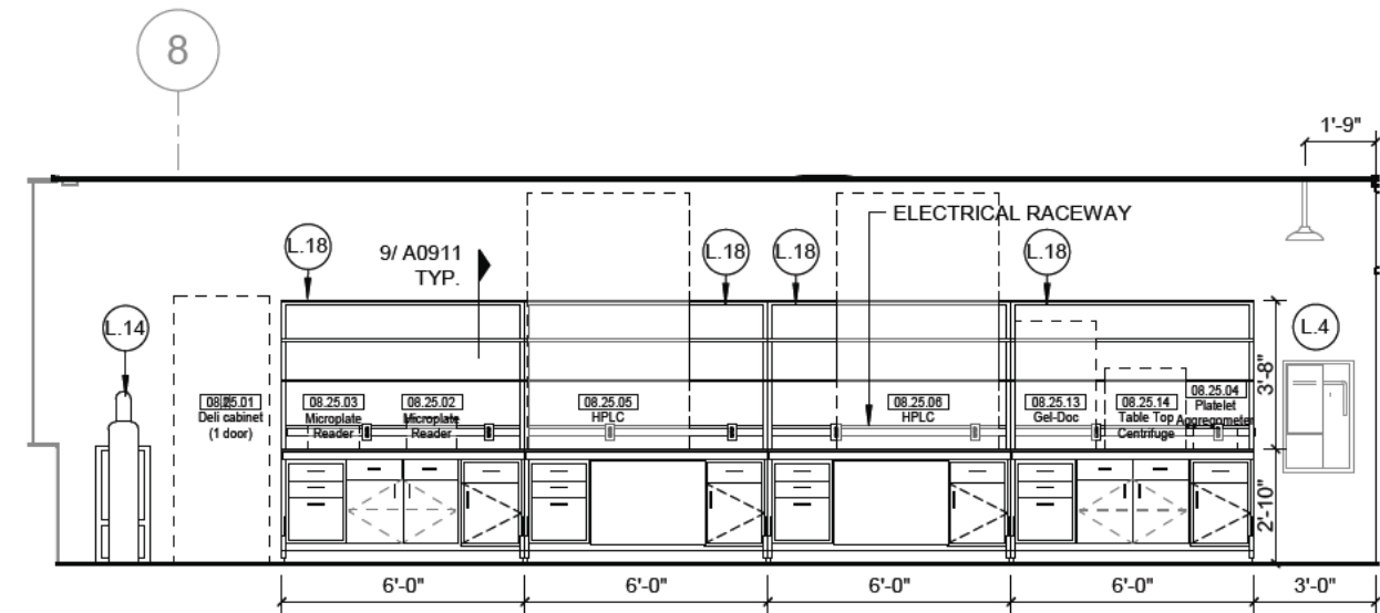
11 L03E BIO FACULTY RESEARCH - NORTH 1/4" = 1'-0"
