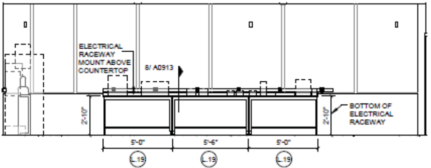
4 L02W MICRO / PLANT RESEARCH - WEST 1/4" = 1'-0" REF 1 / A0204
