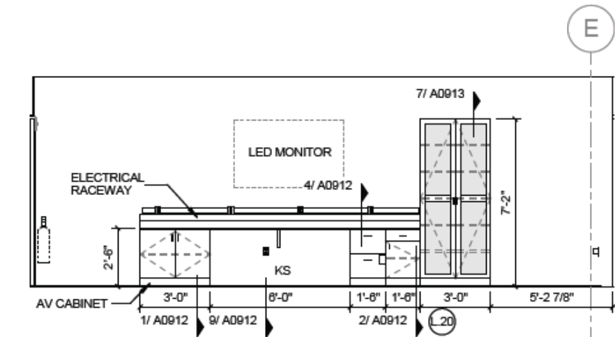
2 L01 CADAVER STORAGE/WORKROOM - WEST 1/4" = 1'-0"
