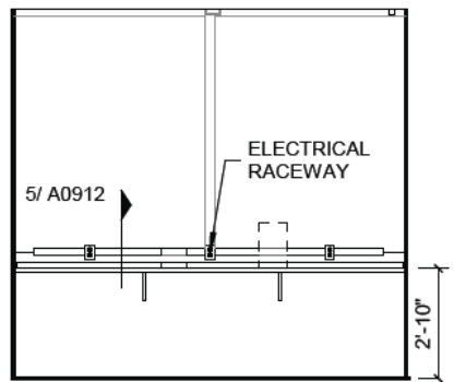
5 L04 CHEMISTRY LAB PREP - EAST 1/4" = 1'-0" REF 2 / A0207
