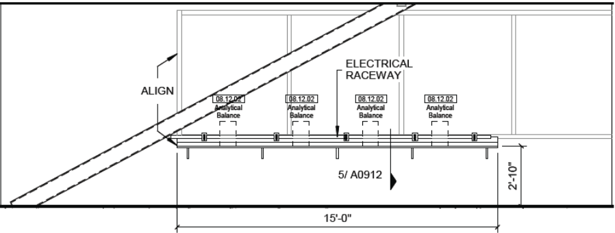
15 L04 ANALYTICAL/INORGANIC CHEM LAB - EAST 1/4" = 1'-0"
