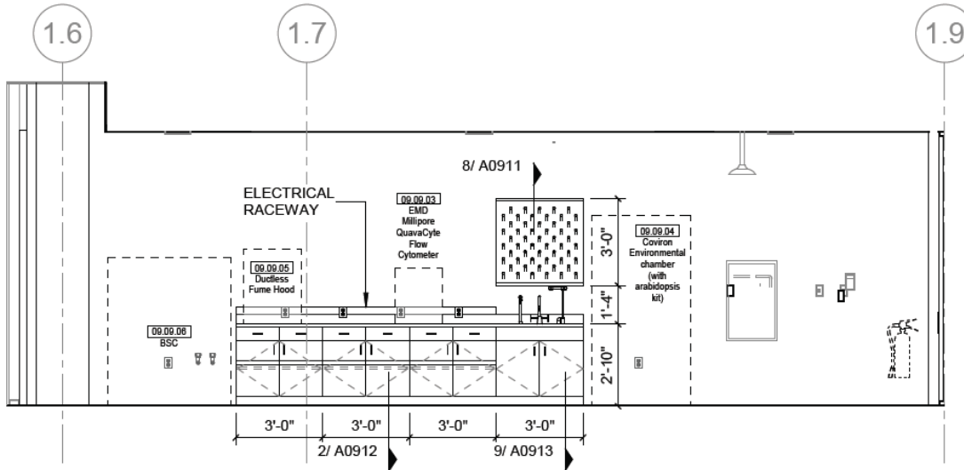
17 L02 OPEN RESEARCH LAB - TABLES - NORTH & SOUTH ELEVATION 1/4" = 1'-0"
