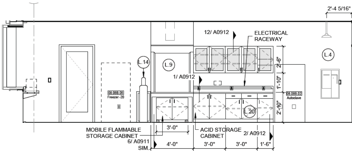
4 L03E BIO LAB PREP 8.08B - SOUTH 1/4" = 1'-0"
