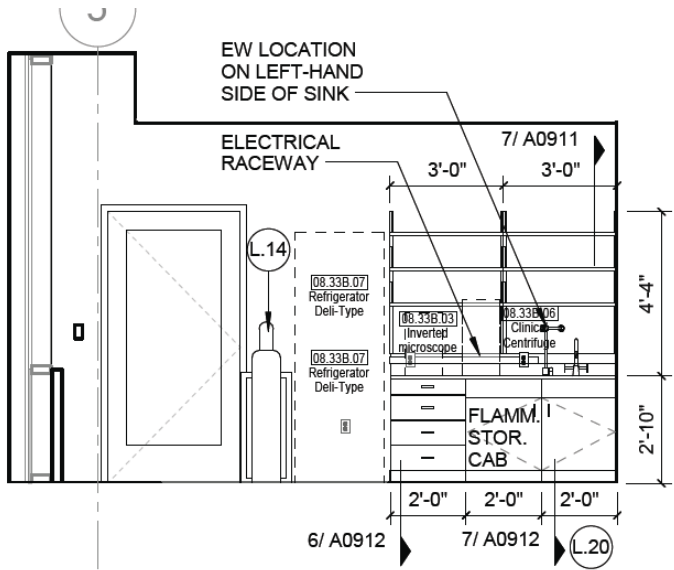
7 L02 TISSUE CULTURE - NORTH 1/4" = 1'-0"
