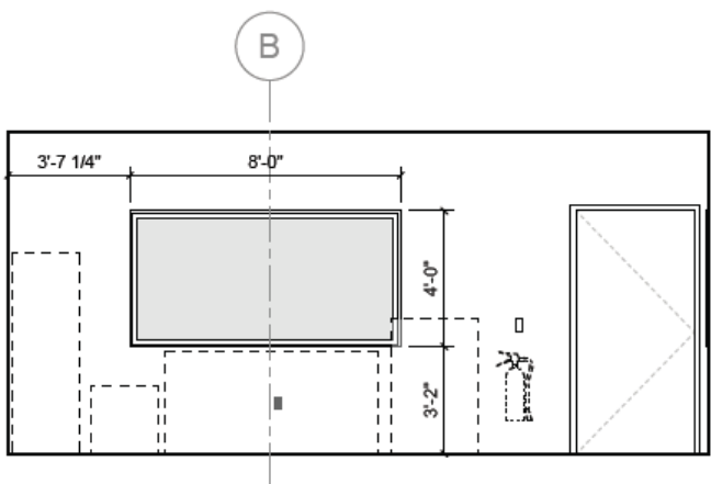
12 L01 SIM LAB - EAST 1/4" = 1'-0"
