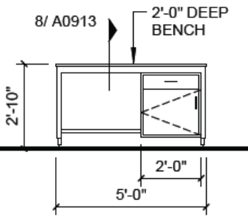
12 TYPICAL TEACHING BENCH 1/4" = 1'-0"
