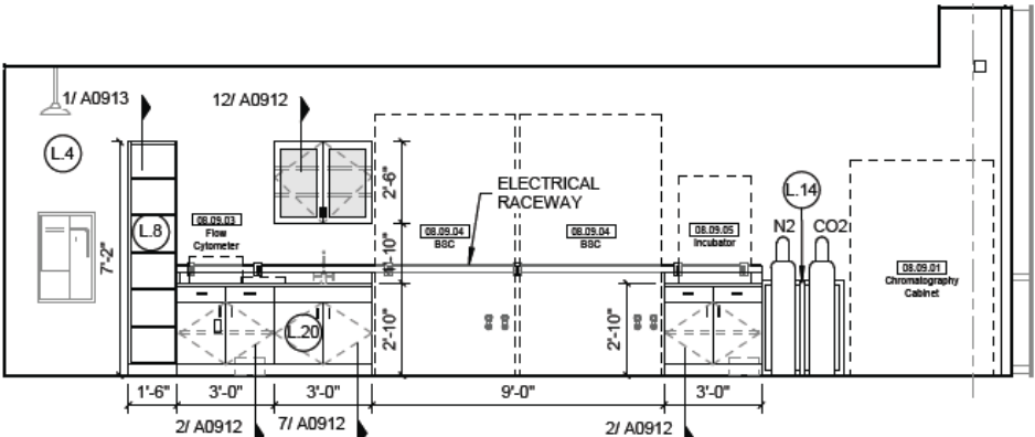
1 L03 CELL BIO / BIOCHEM LAB - SOUTH 1/4" = 1'-0"
