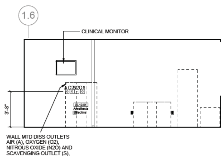
9 L01 SIM LAB - NORTH 1/4" = 1'-0"
