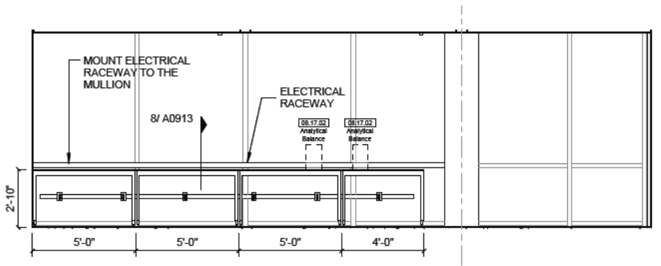
11 L04 PHYSICAL CHEMISTRY LAB - WEST 1/4" = 1'-0"
