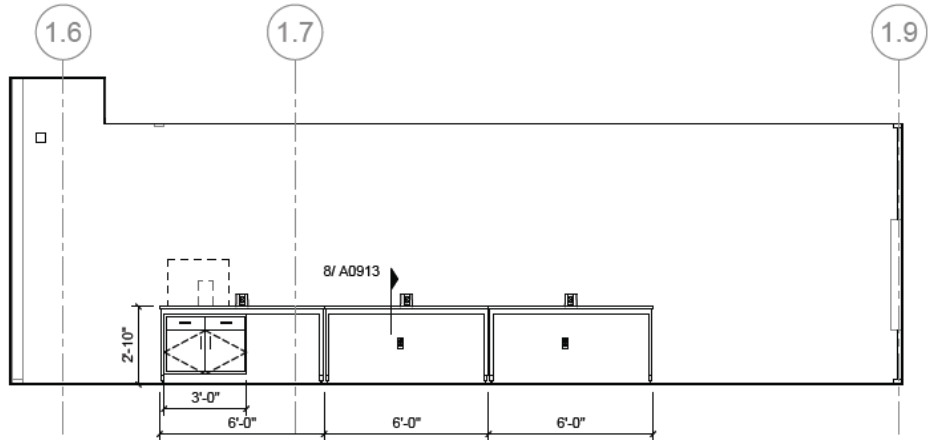
17 L02 OPEN RESEARCH LAB - TABLES - NORTH & SOUTH ELEVATION 1/4" = 1'-0"
