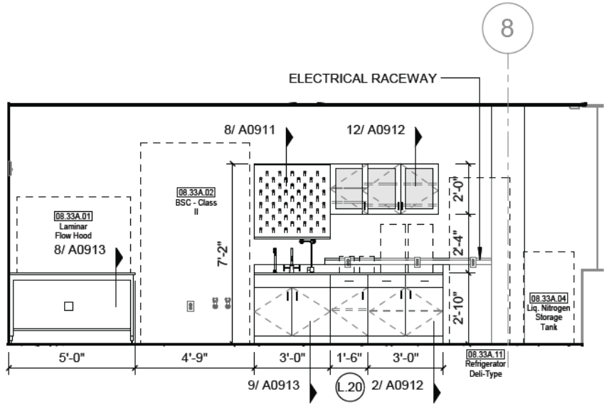
13 L03E TISSUE CULTURE - NORTH 1/4" = 1'-0"
