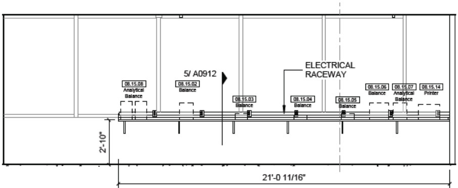
4 L04 GENERAL CHEMISTRY LAB - EAST 1/4" = 1'-0"
