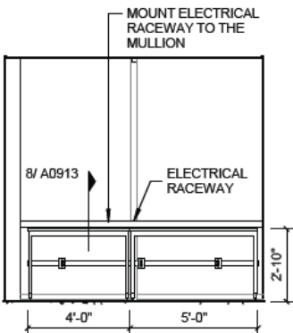
3 L04 INSTRUMENT LAB 8.13 WEST 1/4" = 1'-0"
