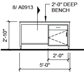
12 TYPICAL TEACHING BENCH 1/4" = 1'-0"
